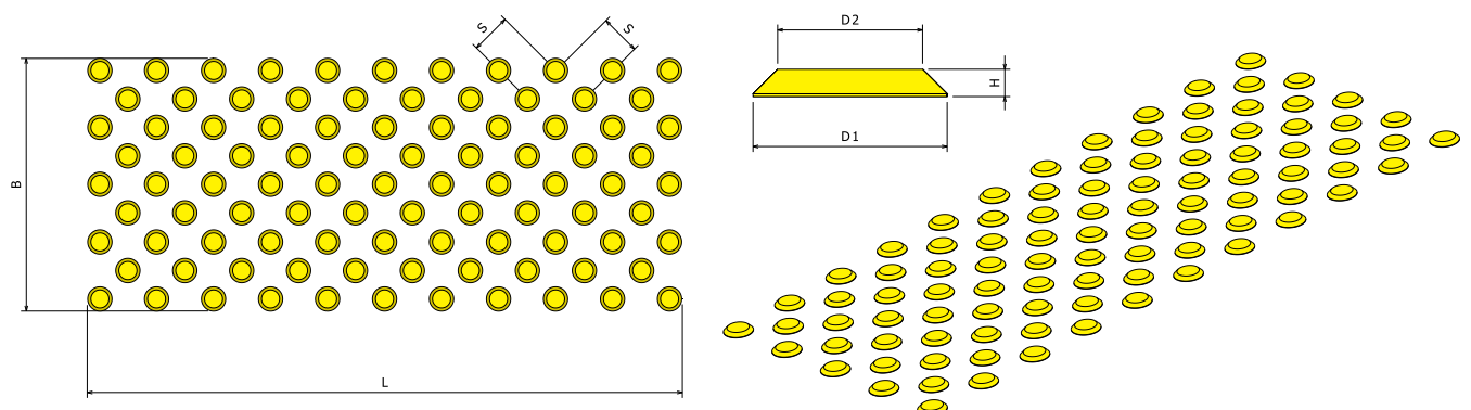
WARNING STUDS IN DIAGONAL ARRANGEMENT, VERTICAL AND ISOMETRIC VIEW
