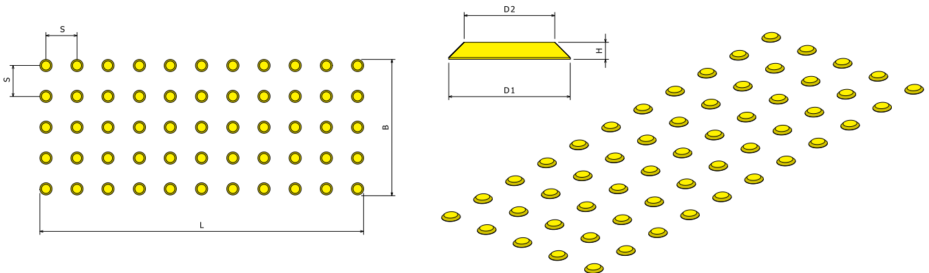
WARNING STUDS IN PARALLEL ARRANGEMENT, VERTICAL AND ISOMETRIC VIEW
